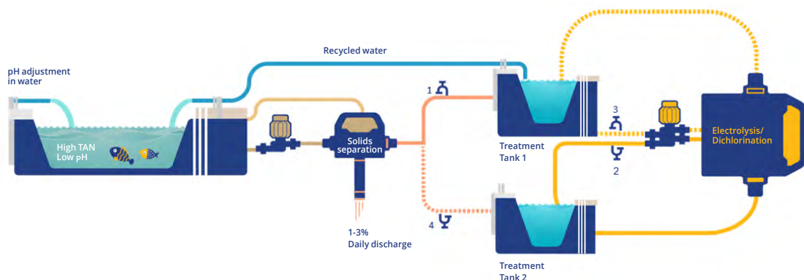
BioFishency ELX – Ammonia Removal and Water Disinfection Process
